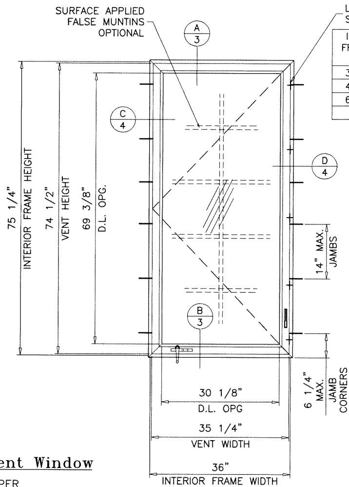
SINGLE VENT (X)
