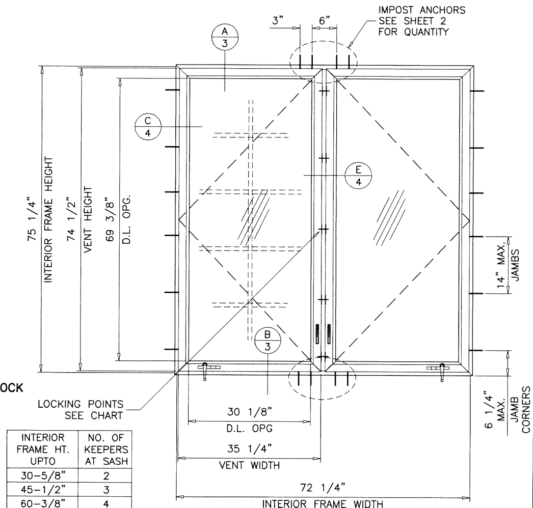
DUAL VENTS (XX)
